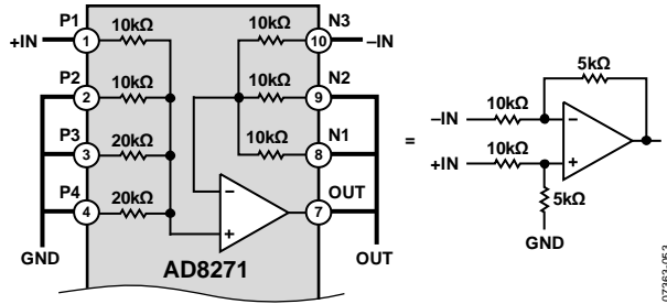
Figure 45. Gain = 1/2 Difference Amplifier, Referenced to Ground
