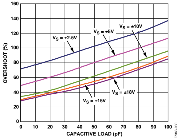
Figure 28. Small-Signal Overshoot vs. Capacitive Load, Gain = 1/2
